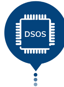
OPERATING SYSTEM
